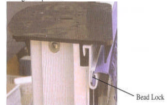
ST031 Rigid Bead Lock 48" long Packaged 48 per case
